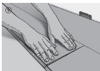
The board is then lowered in on the short side. Ensure here that the board is flush at the short side with the previously laid board. Pressure applied briefly to the side joint clicks in the board.
