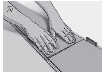
The remaining boards of the first row must be clicked in from above at the head ends into the previous boards. Pressure applied briefly to the side joint clicks in the board into the adjacent board. It is important to ensure that the first row is straight and exactly parallel to the wall. Cut the last board of the first row to size, leaving an expansion gap of 10 - 15 mm (3/8", -1/2") between the board and wall. Fit in the board and lay it flat.
