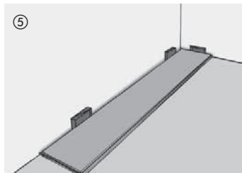
Starting in the right-hand corner of the room, align the boards of the first row with the tongue side parallel to the wall, and fix them in place with wall spacers as you proceed (always keep an expansion gap of 10--15 mm (3/8", -1/2") around perimeter).
