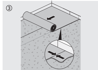
For sound insulation and to smooth out slight irregularities of the subfloor, unroll 2 mm thick cork underlay. Do not overlap. Our range of accessories also offers alternative insulation underlays. Asphalt-bitumen felt is not suitable for sound insulation.
